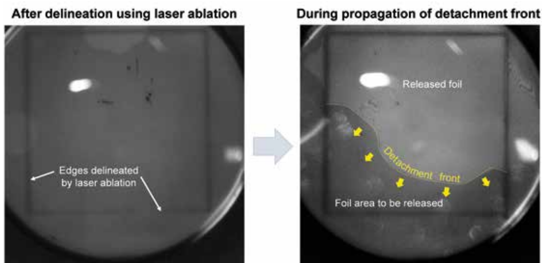
Figure 6. Photoluminescence (PL) images showing the propagation of the detachment front from one edge of the delineated epitaxial Si area to the other edge (the white stains are reflection artefacts).
