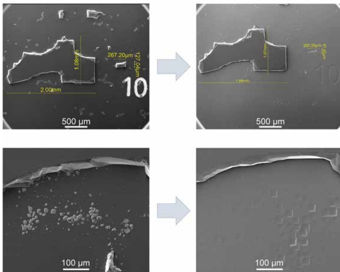
Figure 8. Upon reconditioning by wet chemical etching (here 5μm was removed by TMAH), micrometre-scale defects (such as pillars) are easily dissolved and the surface smoothened out, while larger detachment defects (leading to undetachable epitaxial silicon remnants) remain. Specific markers, such as '10', were used to locate the same region before and after reconditioning.
